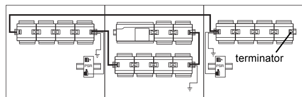
Multisection panel with single length bus
