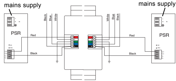
PSR connection to left side PSR connection to right side
